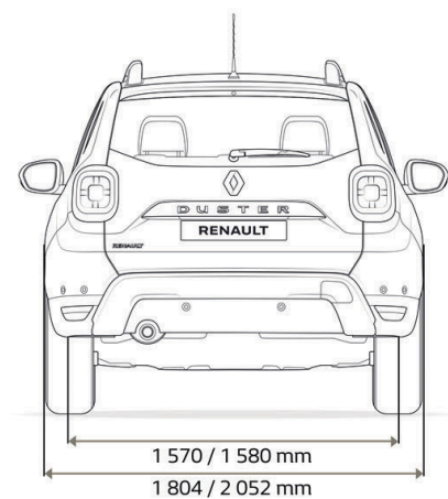
Dimensions (mm)
